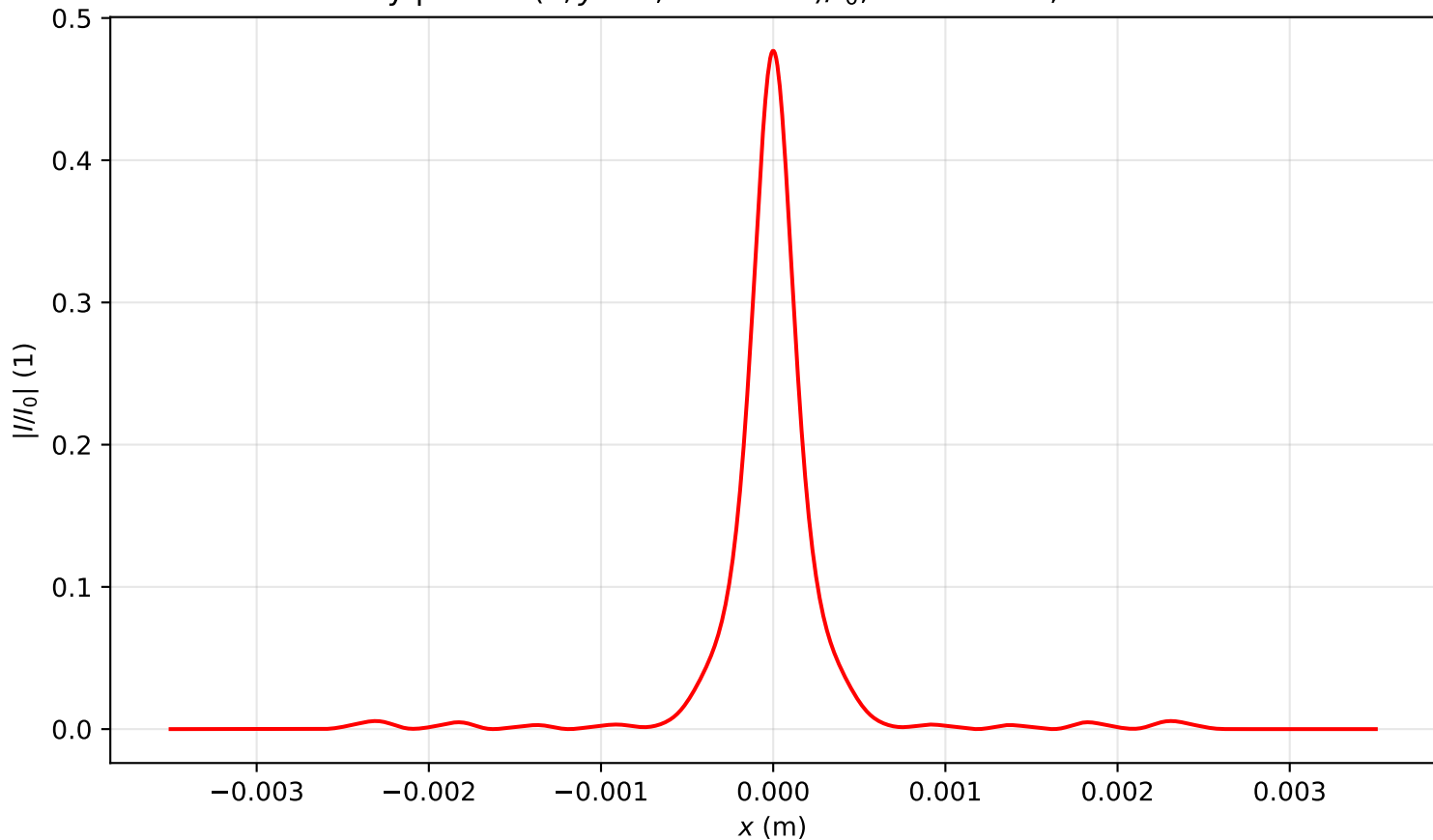
Intensity profile I(x, y = 0, z = 3.184)/I_0 , P_{in}=7.0P_{cr} , artificial time
